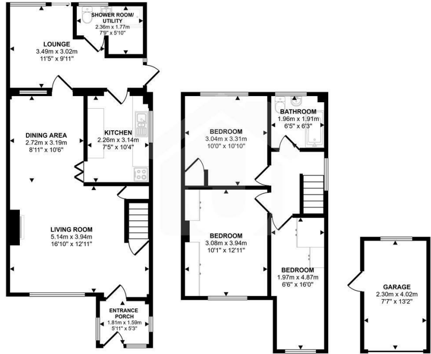
Ground Floor Approx 56 sq m / 608 sq ft
